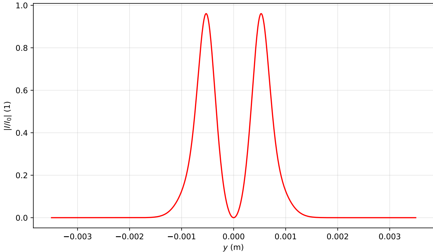
Intensity profile I(x=0, y, z=0.557)/I_0 , P_{in}=4.0P_{cr} , artificial time
